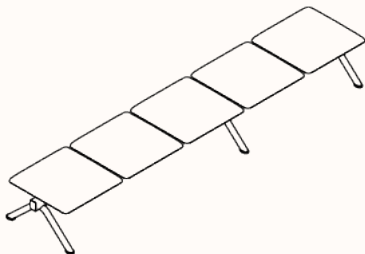
5 Seat Bench OW 3075mm OD 675mm SH 450mm SD 590mm
