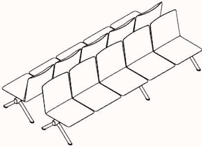
10 Seat Back to Back OW 3075mm OD 1540mm SH 450mm SD 590mm OH 875mm
