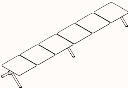
6 Seat Bench OW 3690mm OD 675mm SH 450mm SD 590mm
