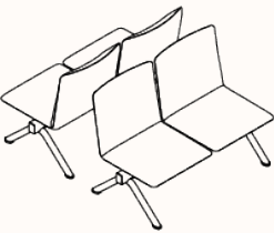
4 Seat Back to Back OW 1230mm OD 1540mm SH 450mm SD 590mm OH 875mm
