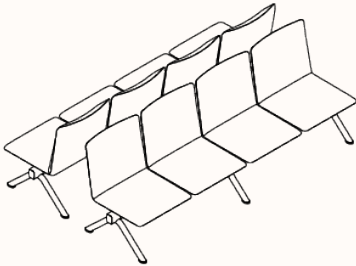
8 Seat Back to Back OW 2460mm OD 1540mm SH 450mm SD 590mm OH 875mm
