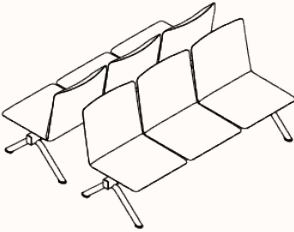
6 Seat Back to Back OW 1845mm OD 1540mm SH 450mm SD 590mm OH 875mm
