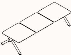
3 Seat Bench OW 1845mm OD 675mm SH 450mm SD 590mm
