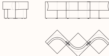
Congif. 6.3 367.112.Z4.B63 OW 2780mm OD 1080mm OH 720mm SH 400mm
