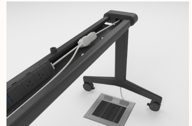
Cable Leg Detail
