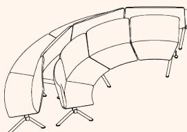
Curved 120 Back to Back OW 4530mm OD 2080mm SH 450mm SD 480mm OH 875mm External Radius: 2635mm
