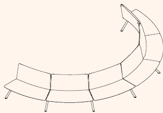
Convex 180 OW 5280mm OD 2640mm SH 450mm SD 480mm OH 875mm External Radius: 2635mm
