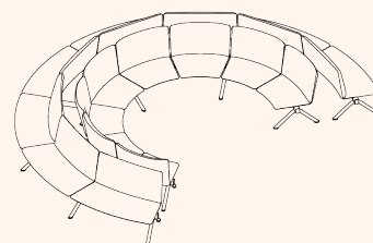
Curved 240 Back to Back OW 5280mm OD 3935mm SH 450mm SD 480mm OH 875mm External Radius: 2635mm
