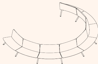
Convex 240 OW 5280mm OD 3935mm SH 450mm SD 480mm OH 875mm External Radius: 2635mm
