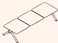
3 Seat Bench OW 1845mm OD 675mm SH 450mm SD 590mm
