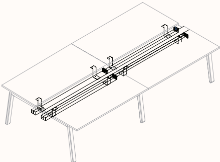
180 Degree Pod of 4 with 96mm Duct
