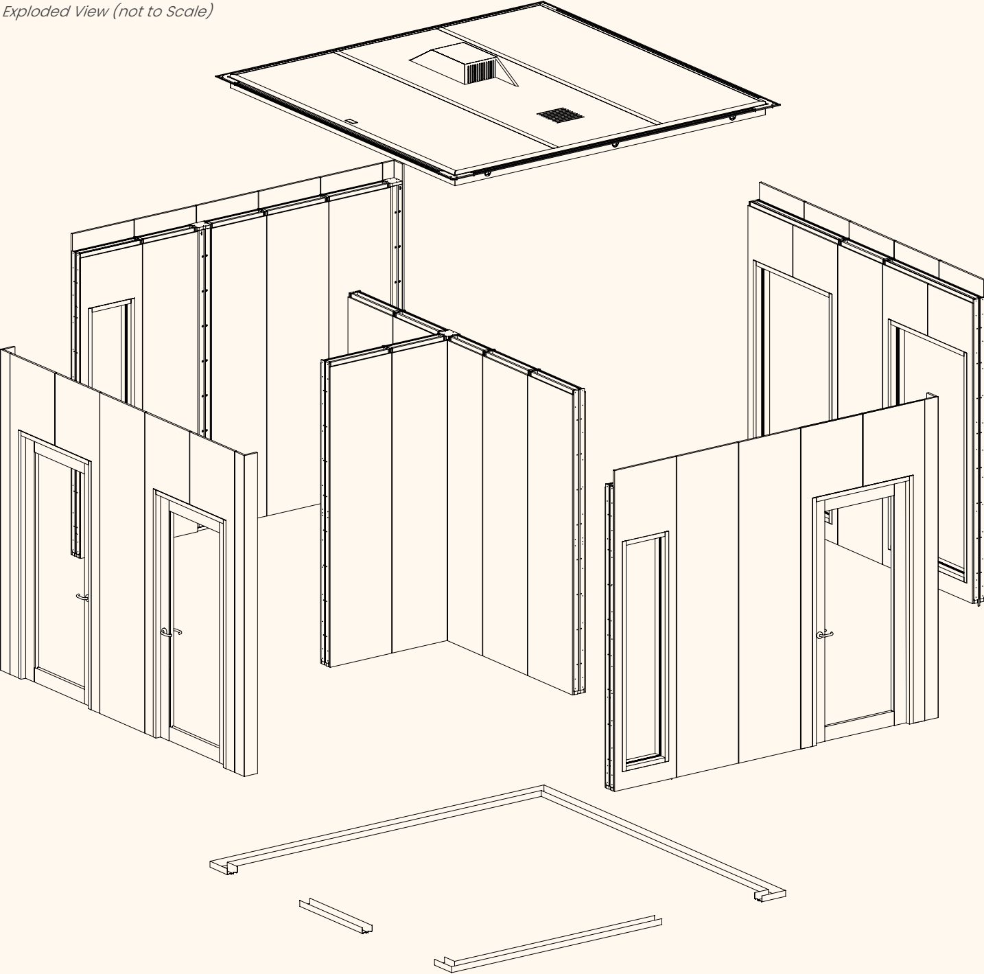
Exploded View (not to Scale)
