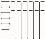
Lounge Large Short Armrest Right OW 1530mm OD 1300mm SH 470mm SD 1000mm OH 700mm
