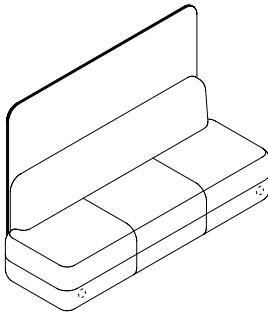
2000 Lounge Module w/ Screen OW 2000mm SD 500mm OD 685mm SH 450mm BH 800mm OH 1200/1375mm
