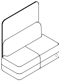
1400 Lounge Module w/ Screen OW 1400mm SD 500mm OD 685mm SH 450mm BH 800mm OH 1200/1375mm
