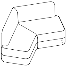
1750 Angled Lounge Module OW 1750mm SD 500mm OD 1040mm SH 450mm OH 800mm
