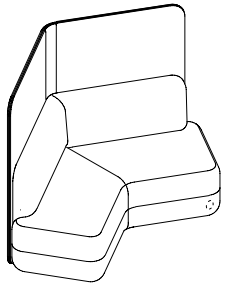
1750 Angled Lounge Module w/ Screen OW 1745mm SD 500mm OD 1070mm SH 450mm BH 800mm OH 1200/1375mm
