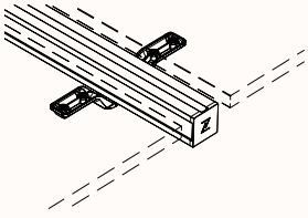
Double Sided Rail (2-Way Handshake Brackets)
